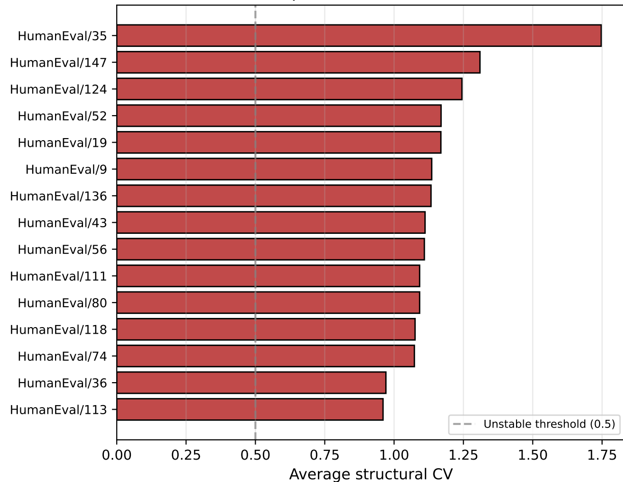
Top 15 most variable tasks (model output inconsistent across runs)
